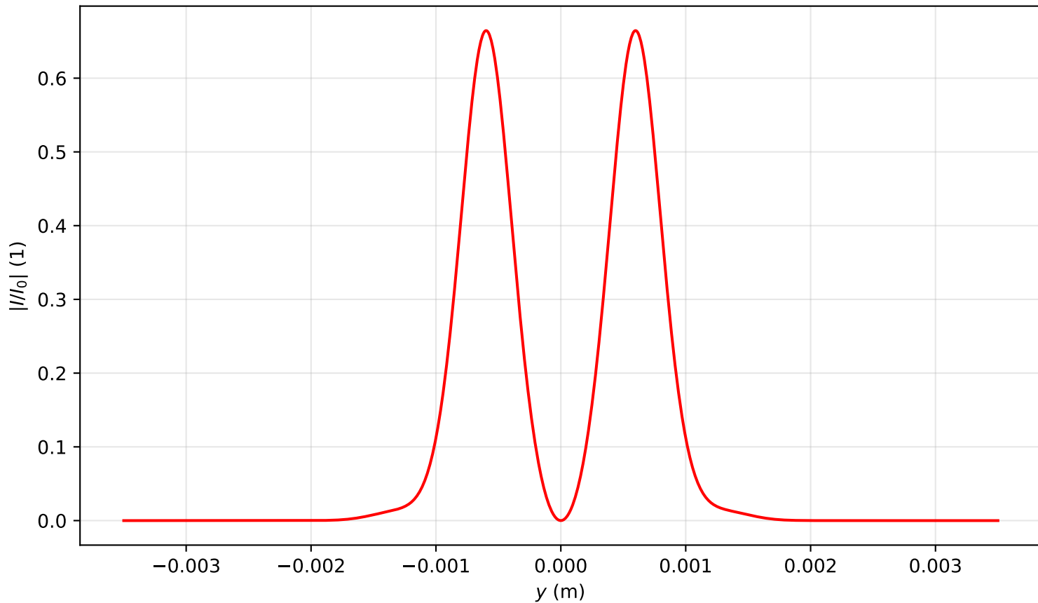
Intensity profile I(x=0, y, z=1.035)/I_0 , P_{in}=3.0P_{cr} , artificial time
